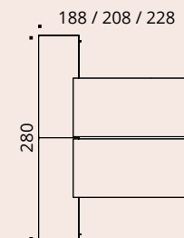
Multi-workstation on B-box console top view
