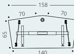
Trapezium end table bottom view
