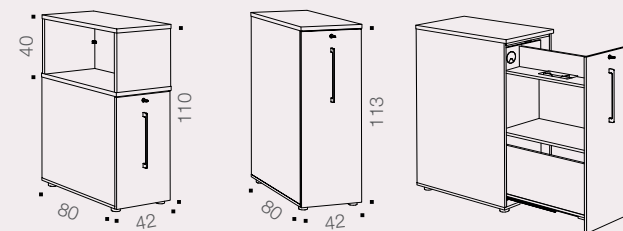
H 110 cm Tower pedestal with Top box
