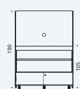
Front view Support TV
